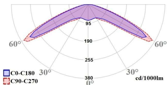
Symmetrical optics
