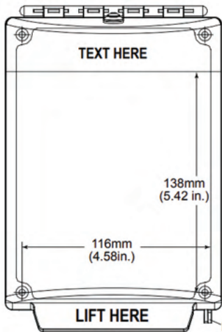
Flush Mount
