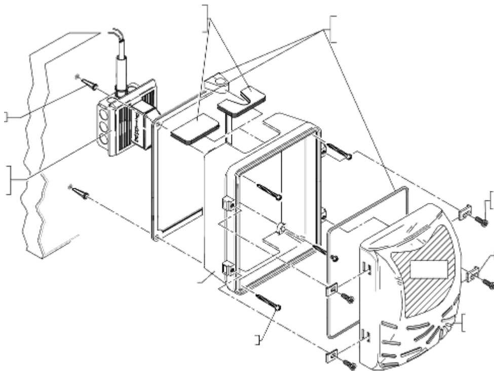
ILLUSTRATON ONLY FOR FS-HS-DS-7135 & FS-HS-DS-8135-PC WITH SURFACE MOUNT SPACER ( D )
