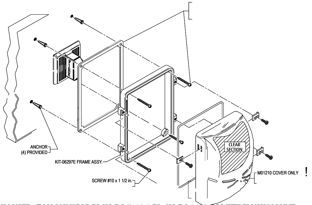
ILLUSTRATON ONLY FOR FS-HS-DS-7125 & FS--HS-DS-8125-PC WITH FLUSH MOUNT SPACER ( E )
