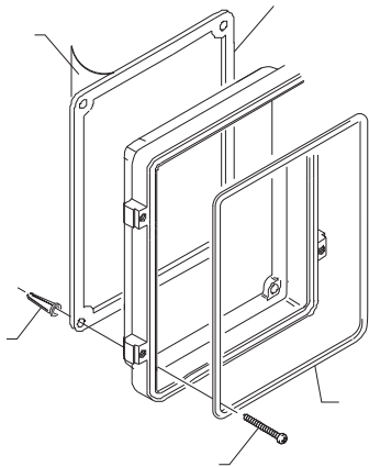
BACK GASKET
