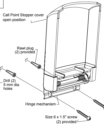
Typical Flush Installation
