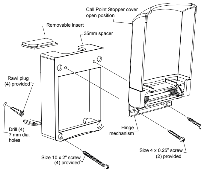
Typical Surface Installation
