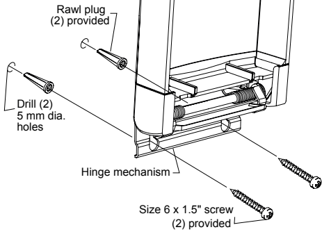
Typical Flush Installation
